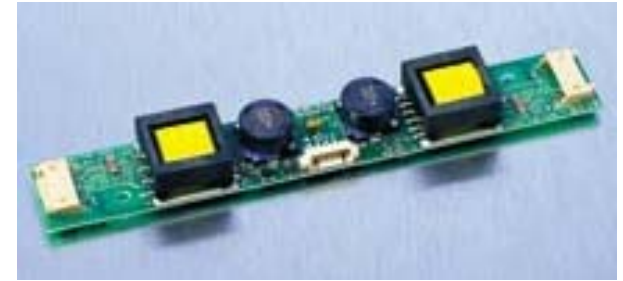
Taiyo Yuden LS520A Inverter
